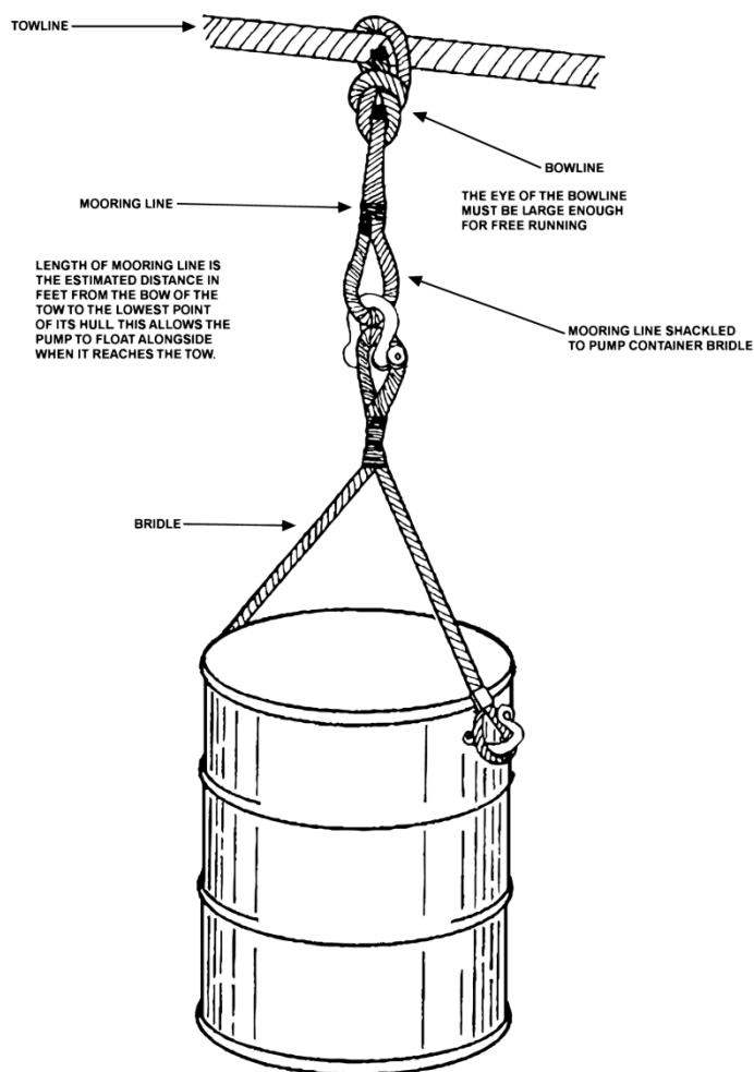
Figure 5-9 Drop Pump on the Towline
