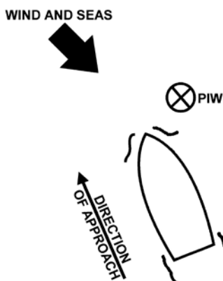
Figure 4-2 Leeward Approach
