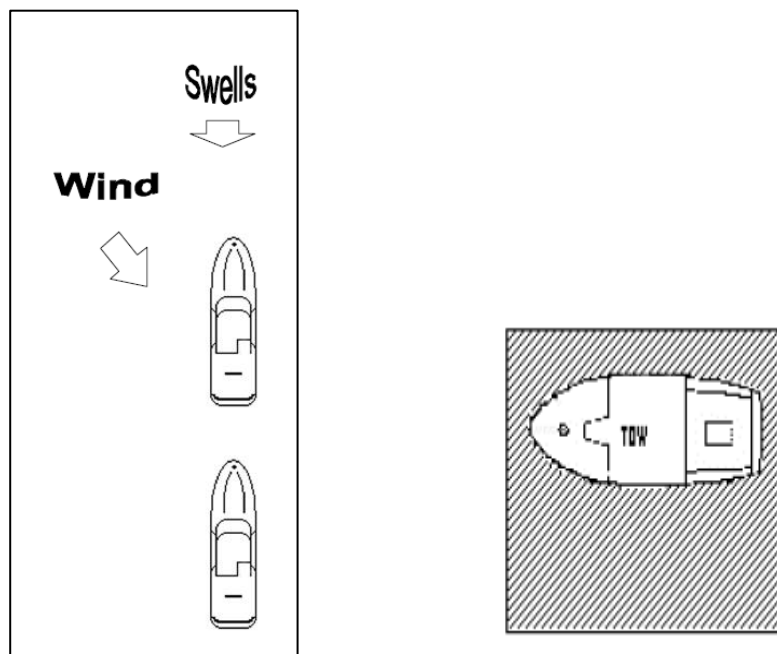
Figure 3-21 Bow-to-Swell Approach
