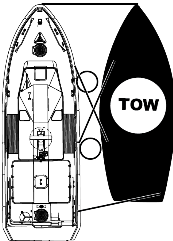
Figure 3-20 Side Tow
