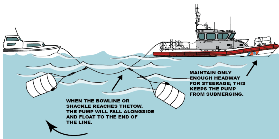
Figure 5-10 Passing a Drop Pump on the Towline
