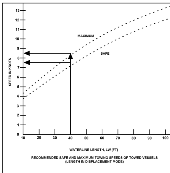
Figure 3-16 Calculated Safe Towing Speeds
