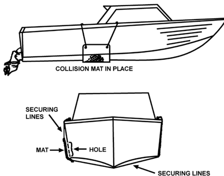
Figure 5-2 Collision Mat
