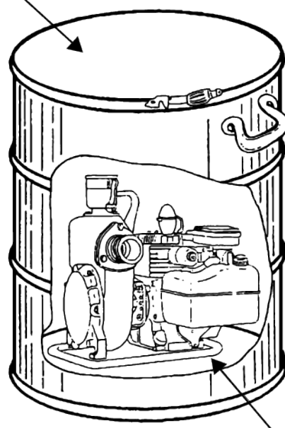
Figure 5-5 Drop Pump
