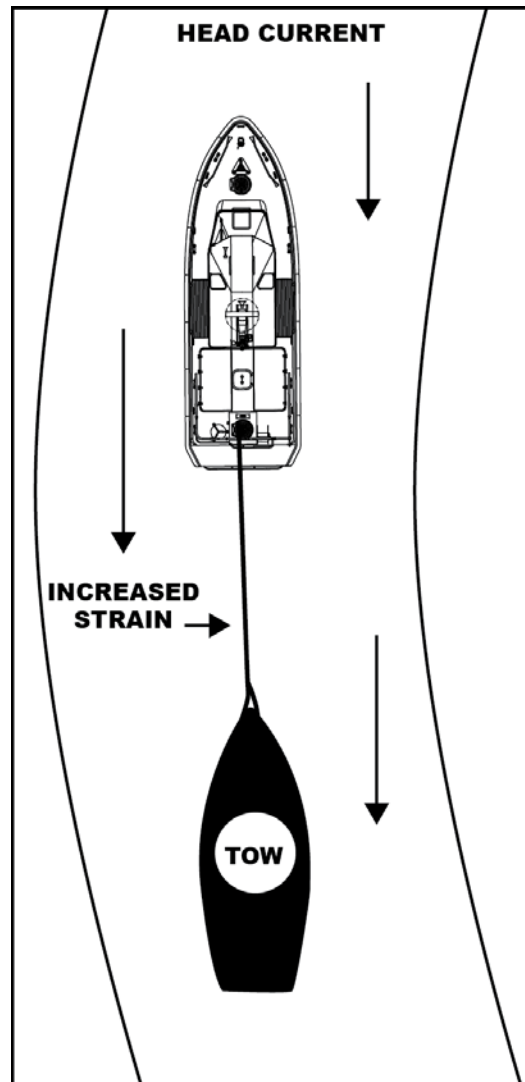
Figure 3-17 Head Current
