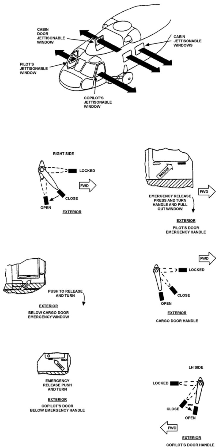
Figure 6-16 MH-60 Emergency Entrances
