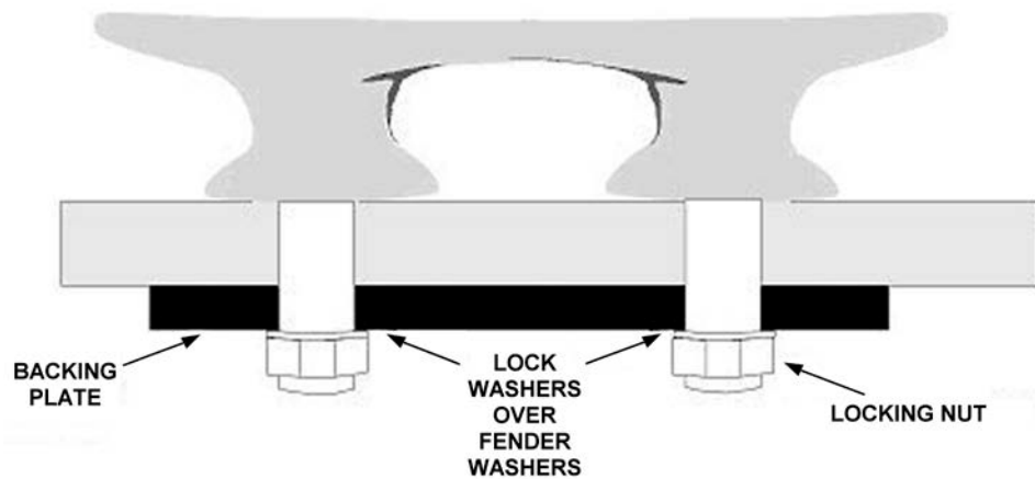
Figure 2-33 Backing Plate
