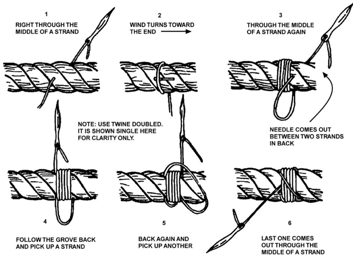
Figure 2-29 Permanent Whipping
