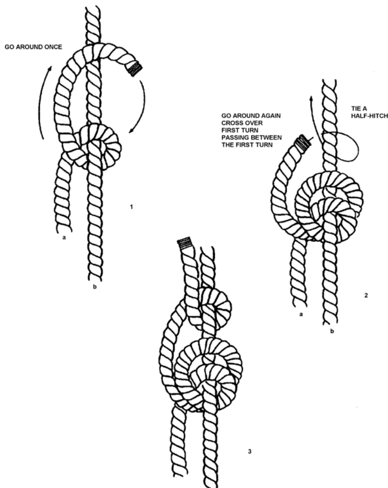
Figure 2-13 Rolling Hitch
