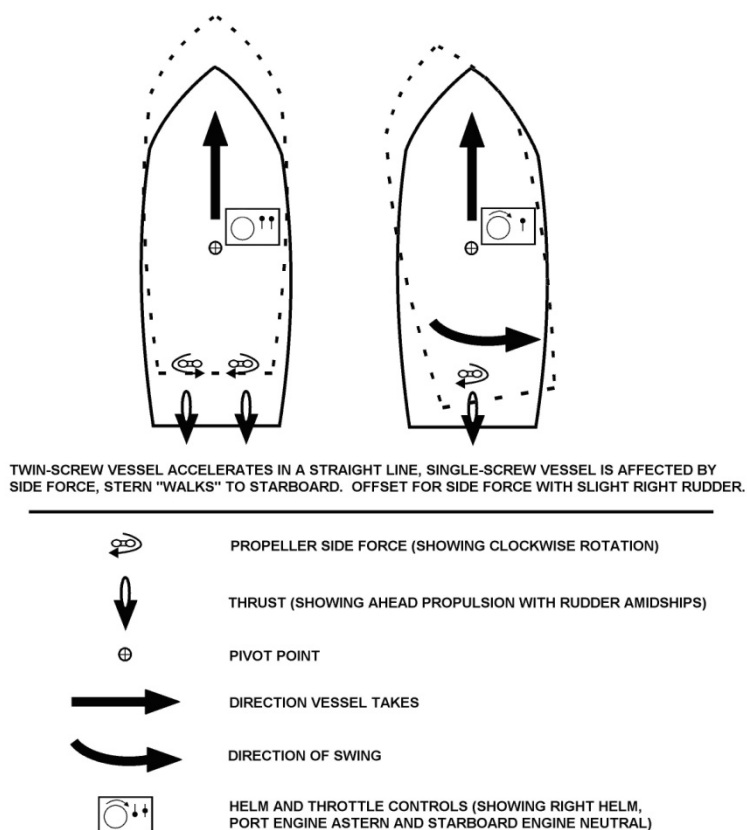
Figure 6-16 Accelerated Ahead
