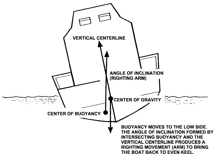
Figure 4-2 Heeling
