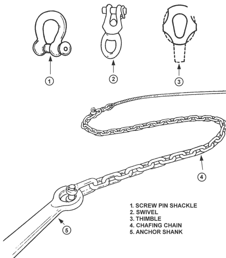
Figure 6-33 Anchor Fittings
