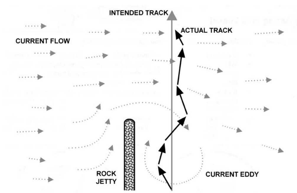
Figure 6-3 Effects of Current
