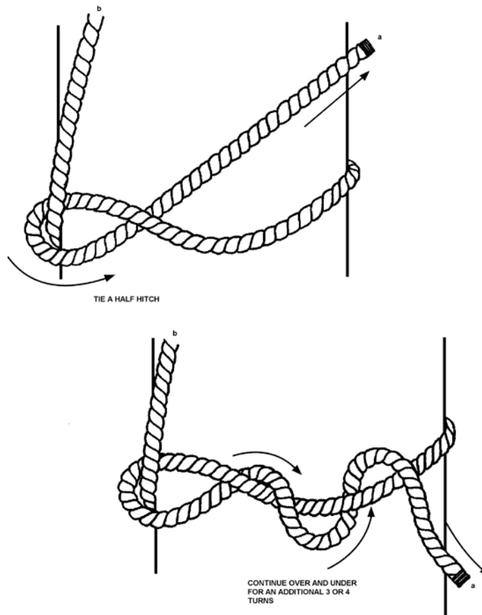
Figure 2-16 Timber Hitch
