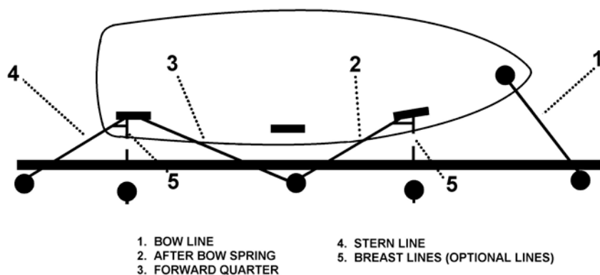
Figure 6-23 Mooring Lines
