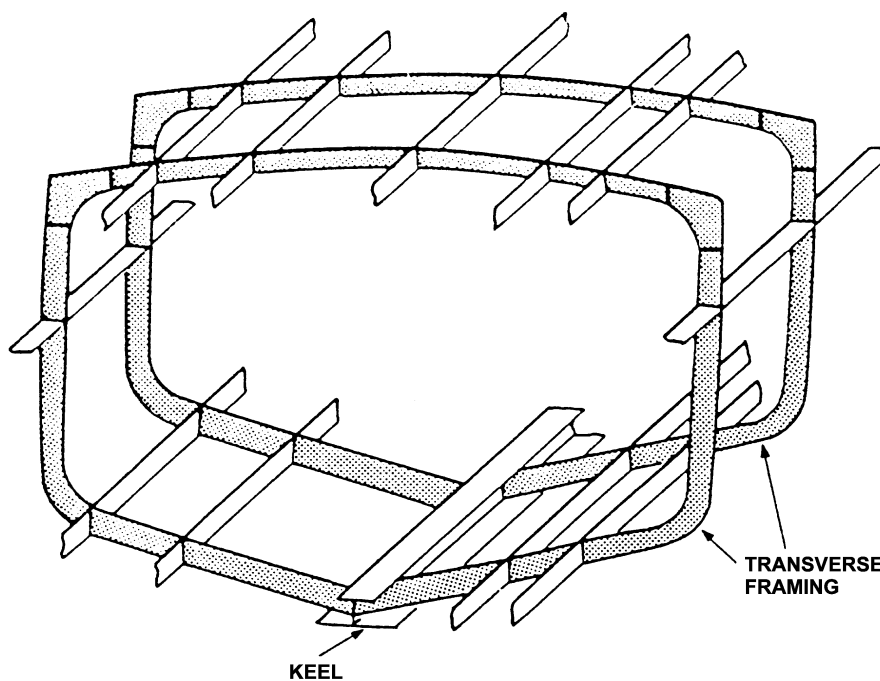
Figure 3-9 Transverse Framing System
