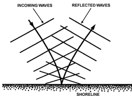
Figure 5-4 Wave Reflection
