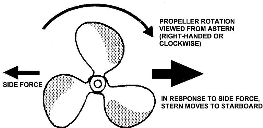
Figure 6-7 Side Force
