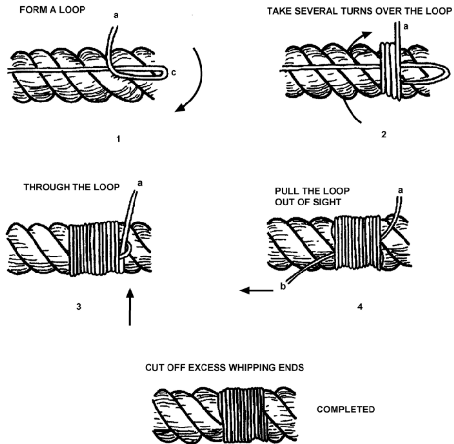
Figure 2-28 Temporary Whipping
