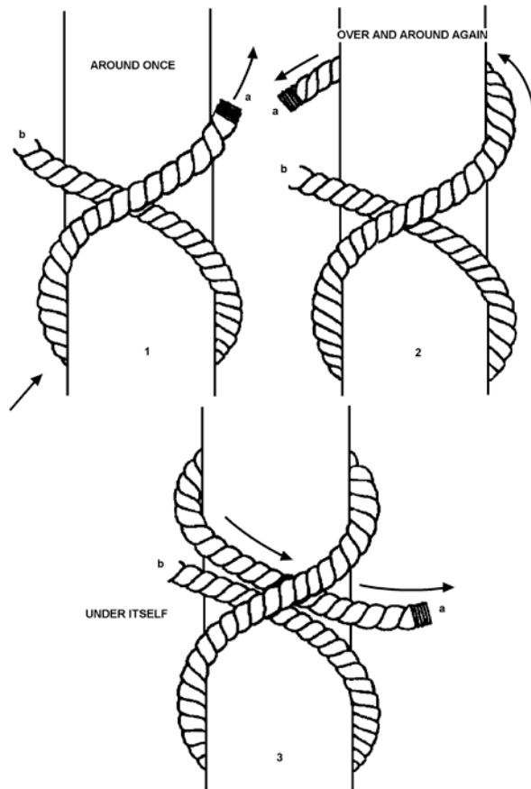
Figure 2-14 Clove Hitch
