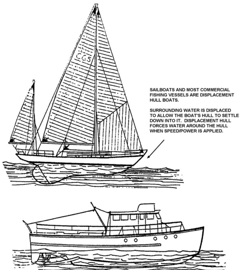
Figure 3-3 Displacement Hulls
