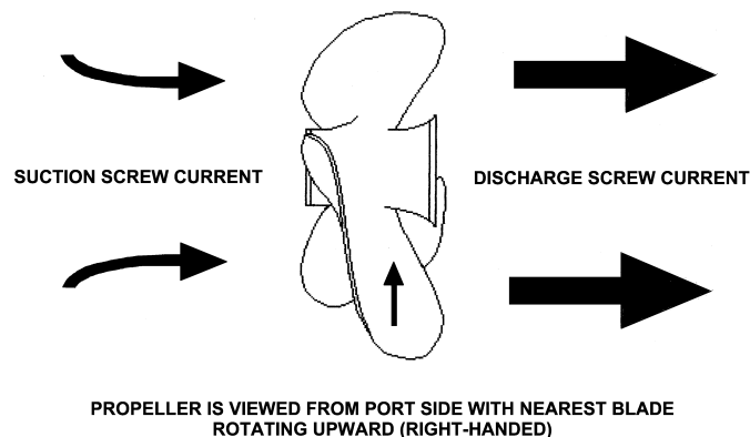
Figure 6-6 Screw Current
