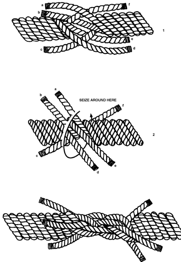
Figure 2-27 Short Splice
